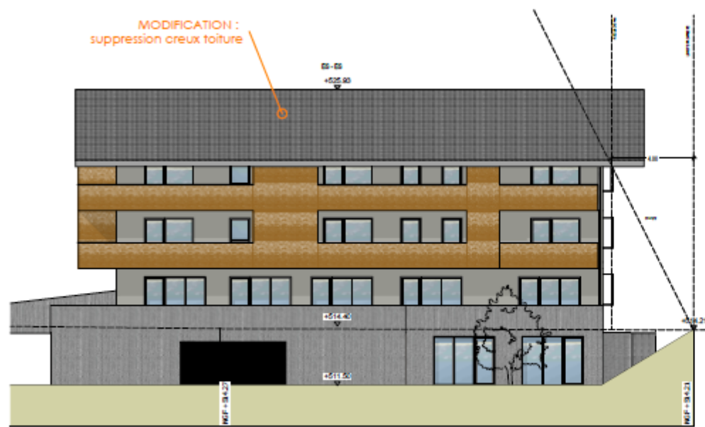
BATIMENT E - FACADE SUD
