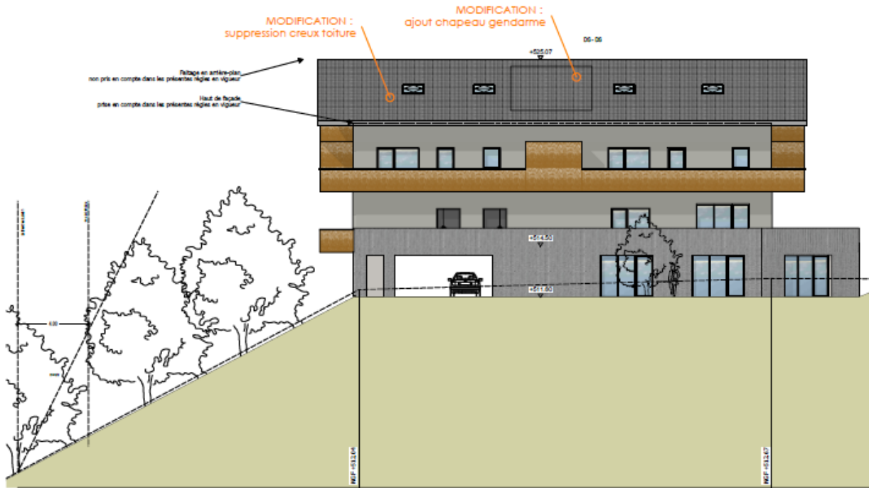
BATIMENT D - FACADE SUD
